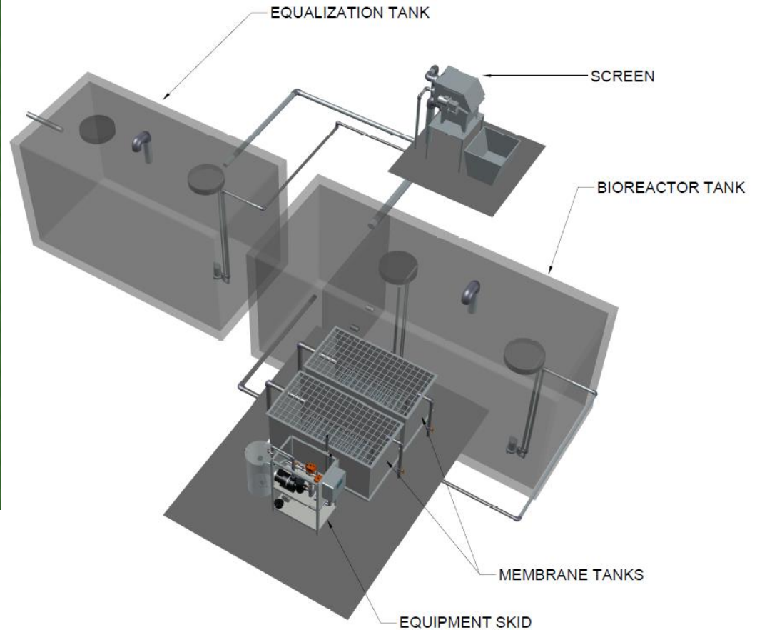
Pictured above: 20,000 GPD nrPUR™ MBR
